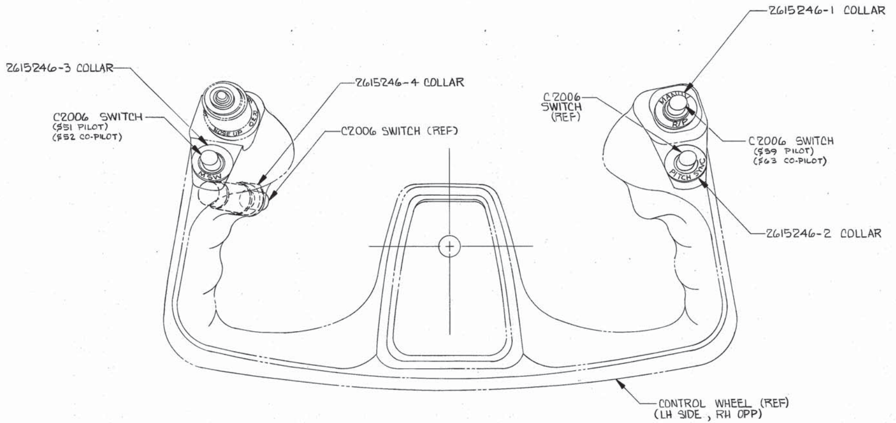
VIEW A-A 41D (LOOKING FWD, LH SIDE SHOWN, RH OPP)
